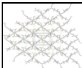
Fig. 2. The crystal packing of (I), viewed along the a axis showing the polymeric structure. Hydrogen bonds are drawn as dashed lines.
