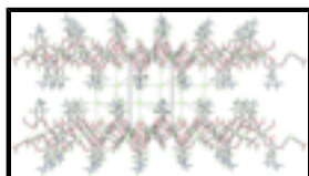
Fig. 3. The crystal packing of (I), viewed along the c axis showing the sheets running along the [010] direction. Hydrogen bonds are drawn as dashed lines.
