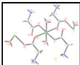
Fig. 1. The structure of (I), showing 50% probability displacement ellipsoids and the atomic numbering. Symmetry codes for the (A) -x, -1/2 + y, -1/2 - z , (B) -x, 1/2 + y, -1/2 - z and (C) -x, -y, -z .
